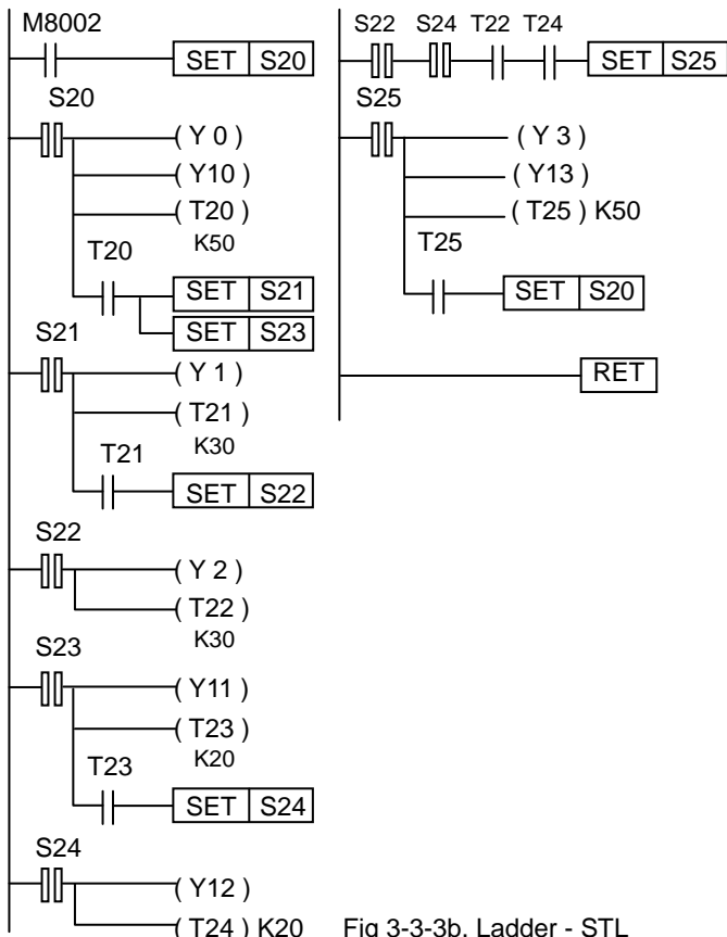
Fig 3-3-3b. Ladder - STL
